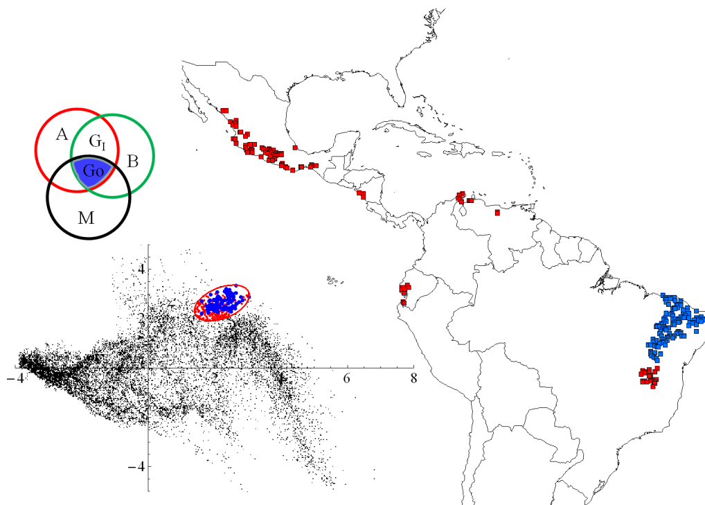
Figure 1. Major symbols used in the paper and their correspondence in geographic and environmental spaces. The first 2 principal components of the environmental space E of the Americas are represented. The Venn diagram is an abstract representation of the geographic space G . The green circle ( B ) represent the regions of the planet that are biologically favorable to the species and the black ( M ) circle the regions that have been accessible to the species over an appropriate period of time. The red circle, in the Venn diagram, symbolized with an A , represents regions with environments within the fundamental niche (the red points inside the ellipse). In the map these correspond to the red and the blue points. In environmental space the existing points inside N_f constitute the existing fundamental niche. The blue points in the map represent those areas that are: i) environmentally favorable, ii) accessible, and iii) biologically suitable. This is the occupied area G_O . Finally, depending on biological suitability, all (or none) of the remaining, unoccupied red points represents a potentially invadable region ( G_I ).
