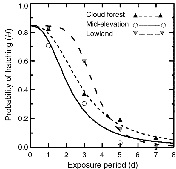
FIG. 4. Decline in hatchability ( H ) of thrasher eggs with exposure, modeled using nonlinear regression forcing the intercept through hatching success (84.3%) for control eggs: H = 0.843 / [1 + a(\text{Exposure})^b] for cloud forest ( a = 0.065 , b = 2.615 , r^2 = 0.59 ), lowland ( a = 0.001 , b = 5.352 , r^2 = 0.689 ), and mid-elevation ( a = 0.141 , b = 2.556 , r^2 = 0.564 ) sites.
